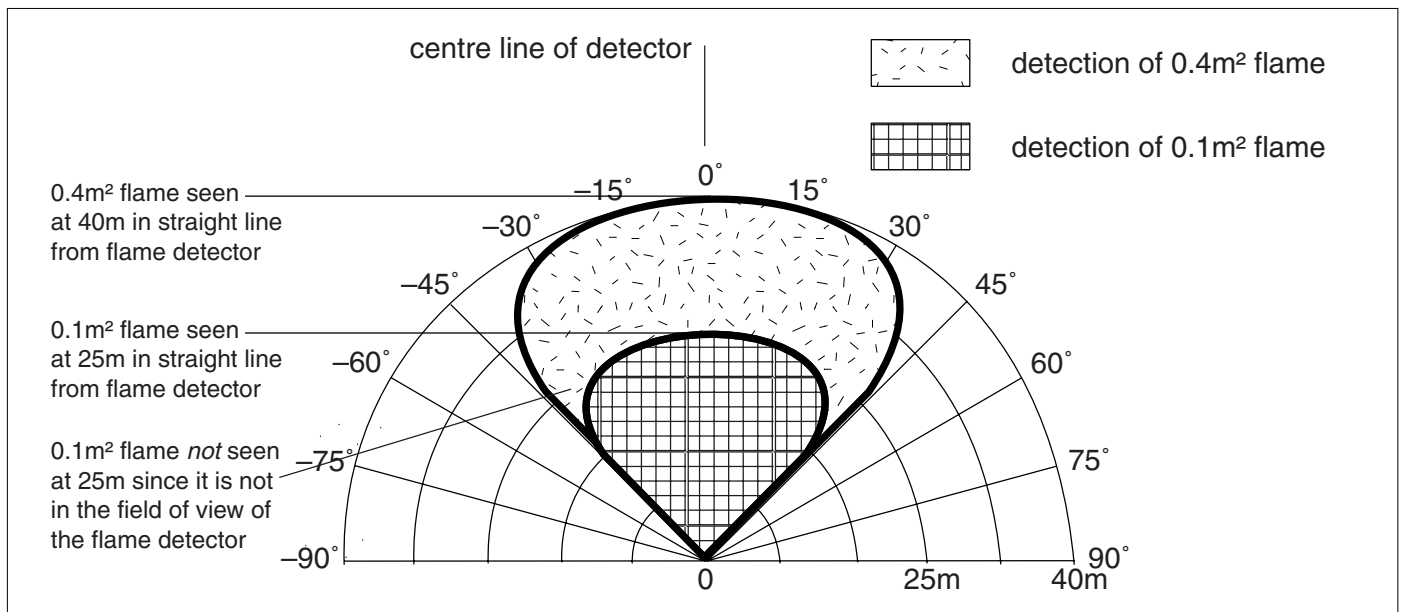
Fig 2 Angle of view of XP95 flame detector
