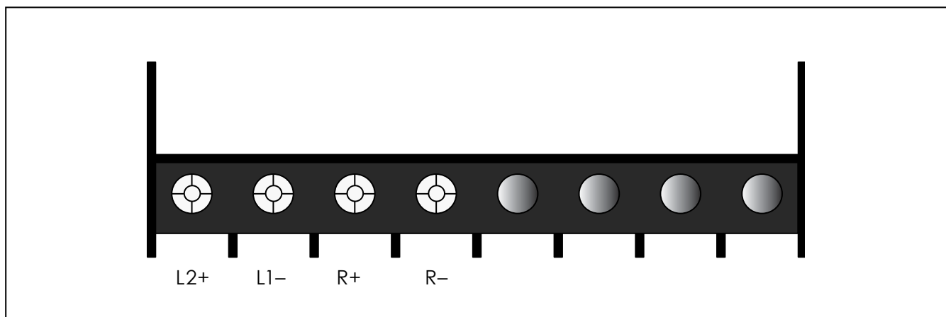
Fig 4 Flame detector wiring connections
