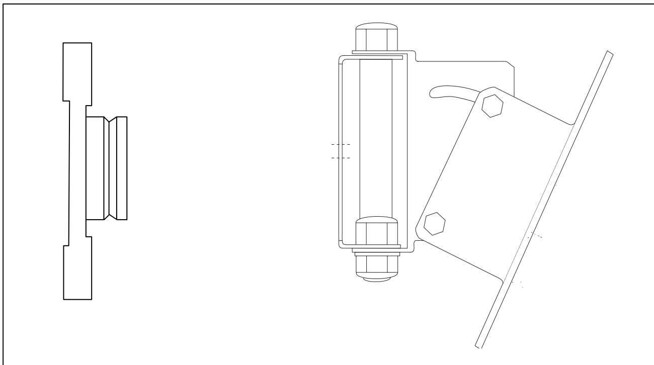
Fig 3 Mounting plate, supplied with detector, and optional adjustable bracket, part no 29600-203
